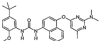
1-(5-tert-Butyl-2-methoxy-phenyl)-3-[4-(2-dimethylamino-6-methyl-pyrimidin-4-yloxy)-naphthalen-1-yl]-urea;
